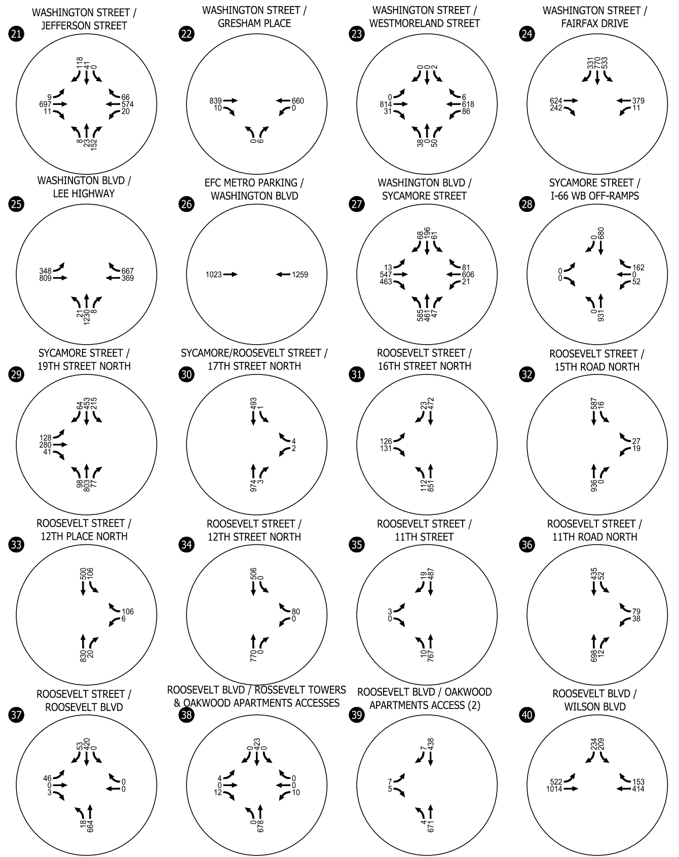
Build Scenario 3 Traffic Volumes Weekday AM Peak Hour
