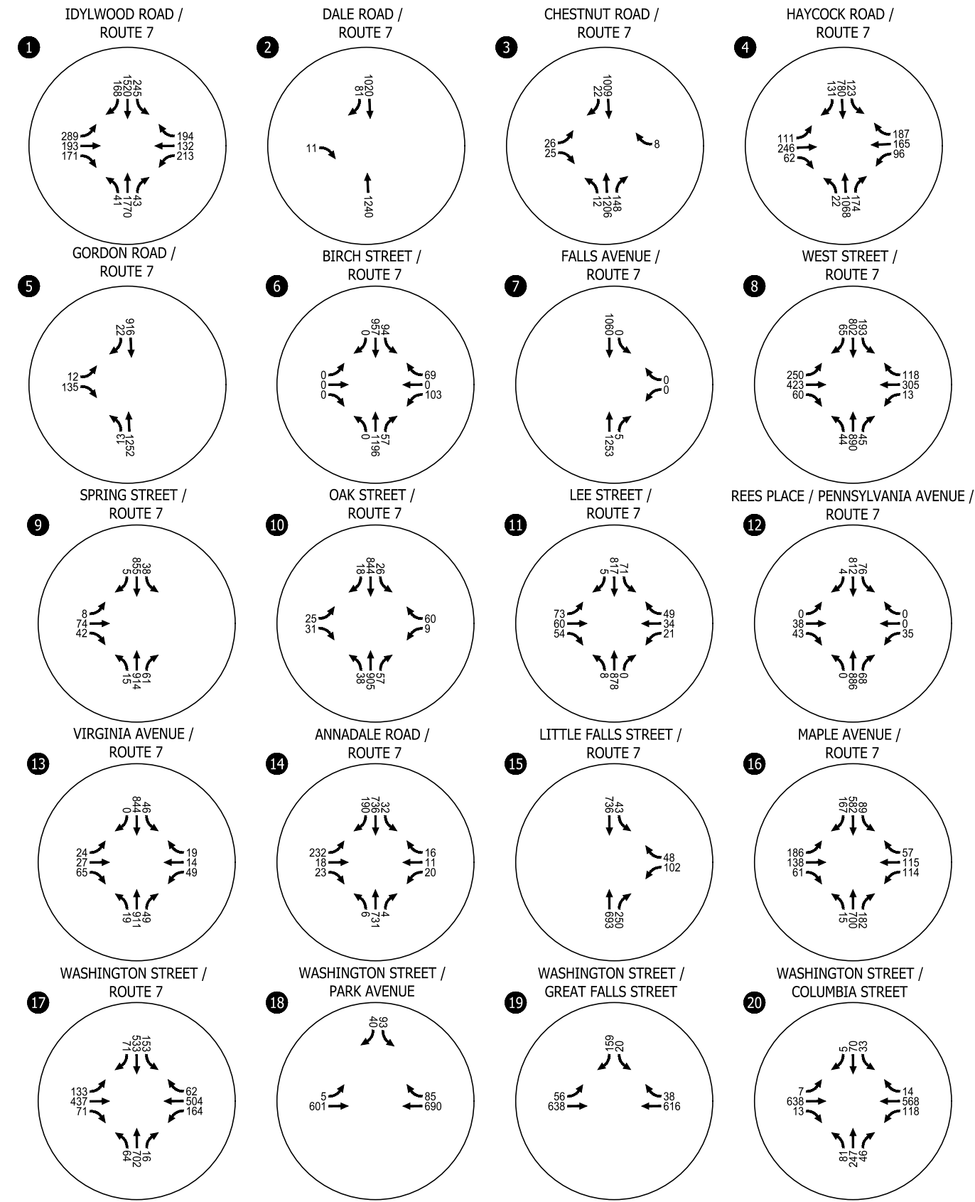
Build Scenario 3 Traffic Volumes Weekday AM Peak Hour
