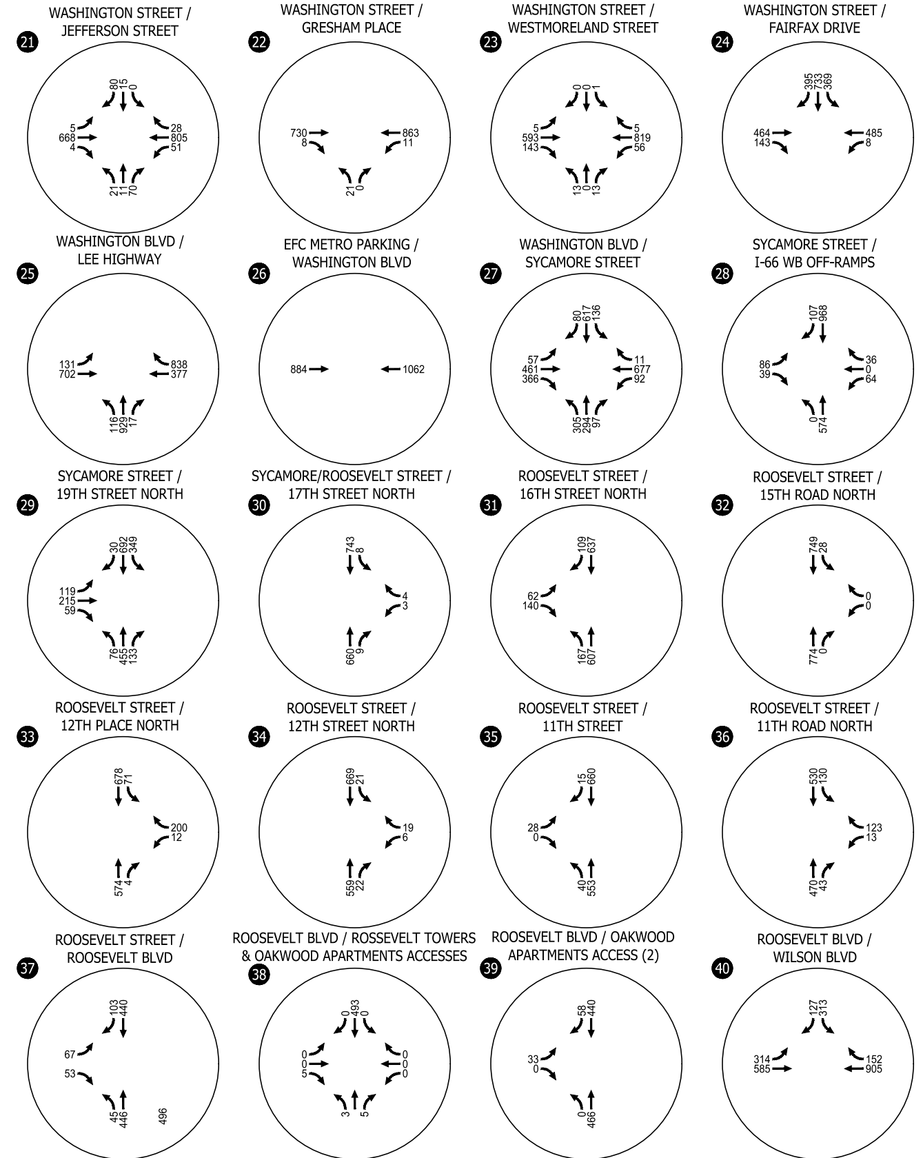
Build Scenario 1 Traffic Volumes Weekday PM Peak Hour
