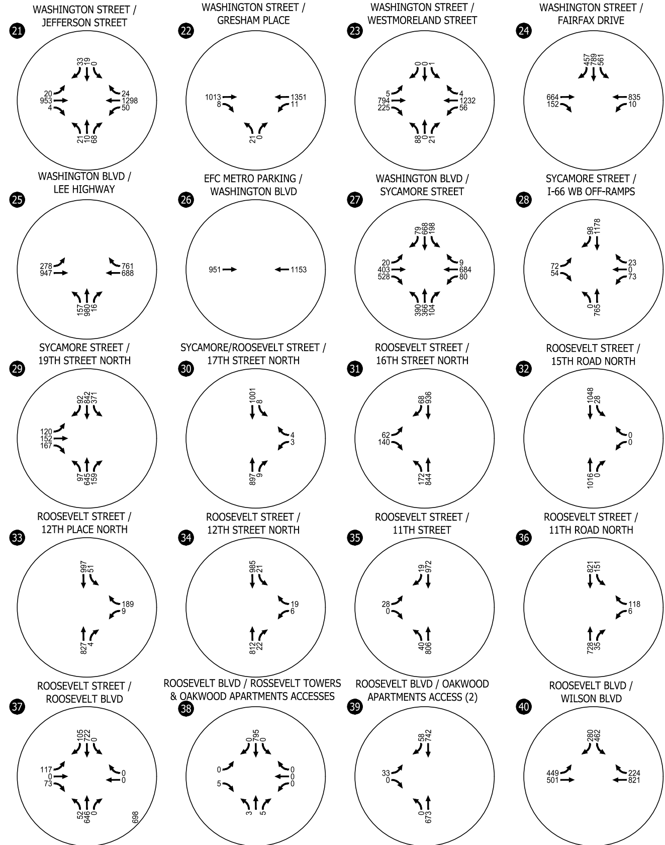
Build Scenario 2 Traffic Volumes Weekday PM Peak Hour
