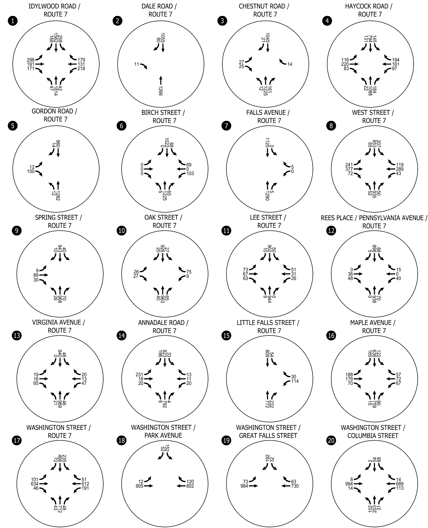
Build Scenario 2 Traffic Volumes Weekday AM Peak Hour
