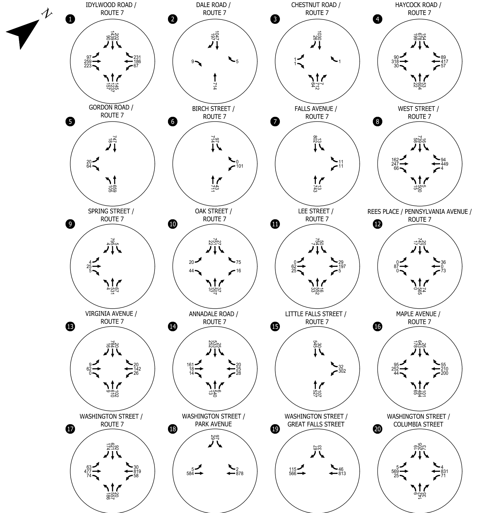
Build Scenario 1 Traffic Volumes Weekday PM Peak Hour
