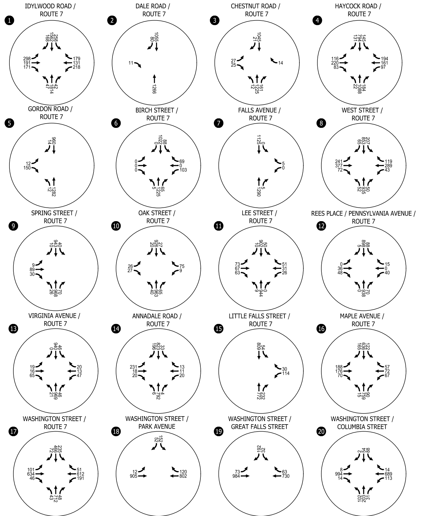
2045 Baseline Traffic Volumes Weekday AM Peak Hour
