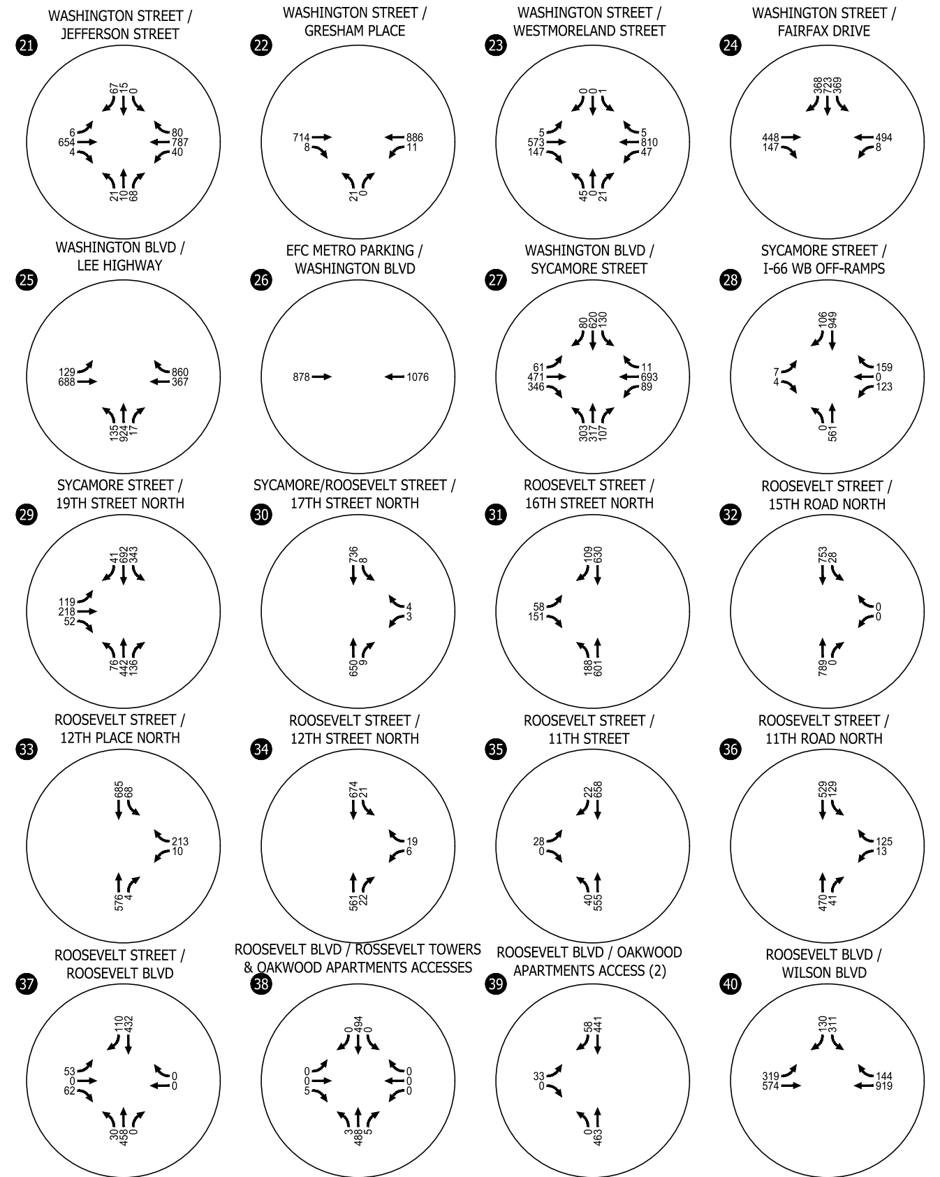
Build Scenario 3 Traffic Volumes Weekday PM Peak Hour
