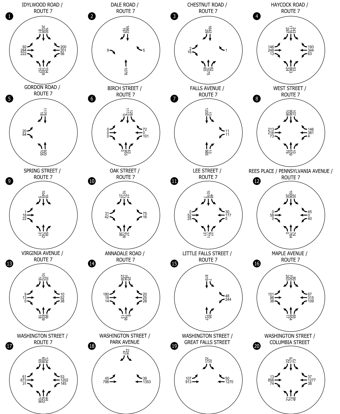
Build Scenario 2 Traffic Volumes Weekday PM Peak Hour
