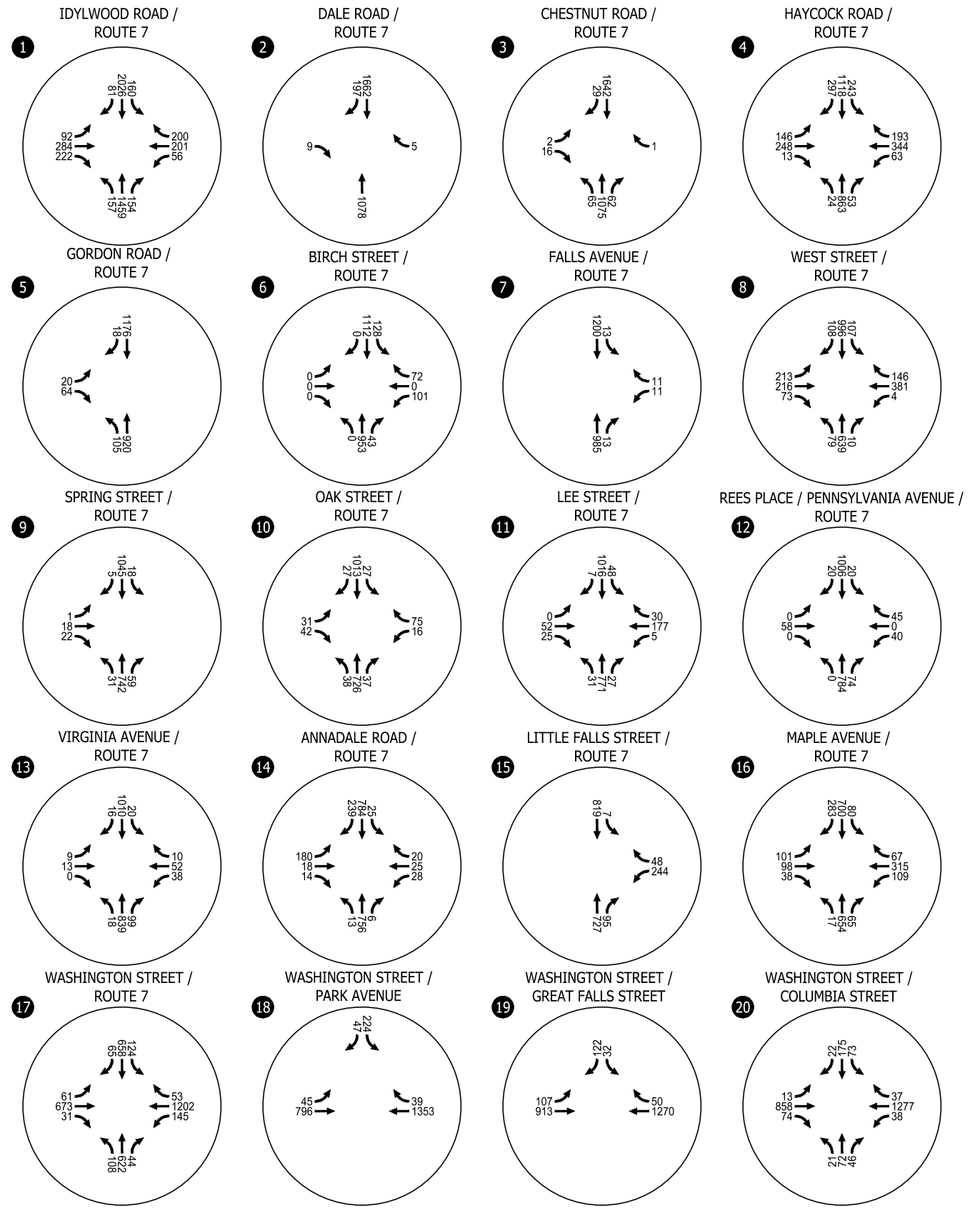
2045 Baseline Traffic Volumes Weekday PM Peak Hour
