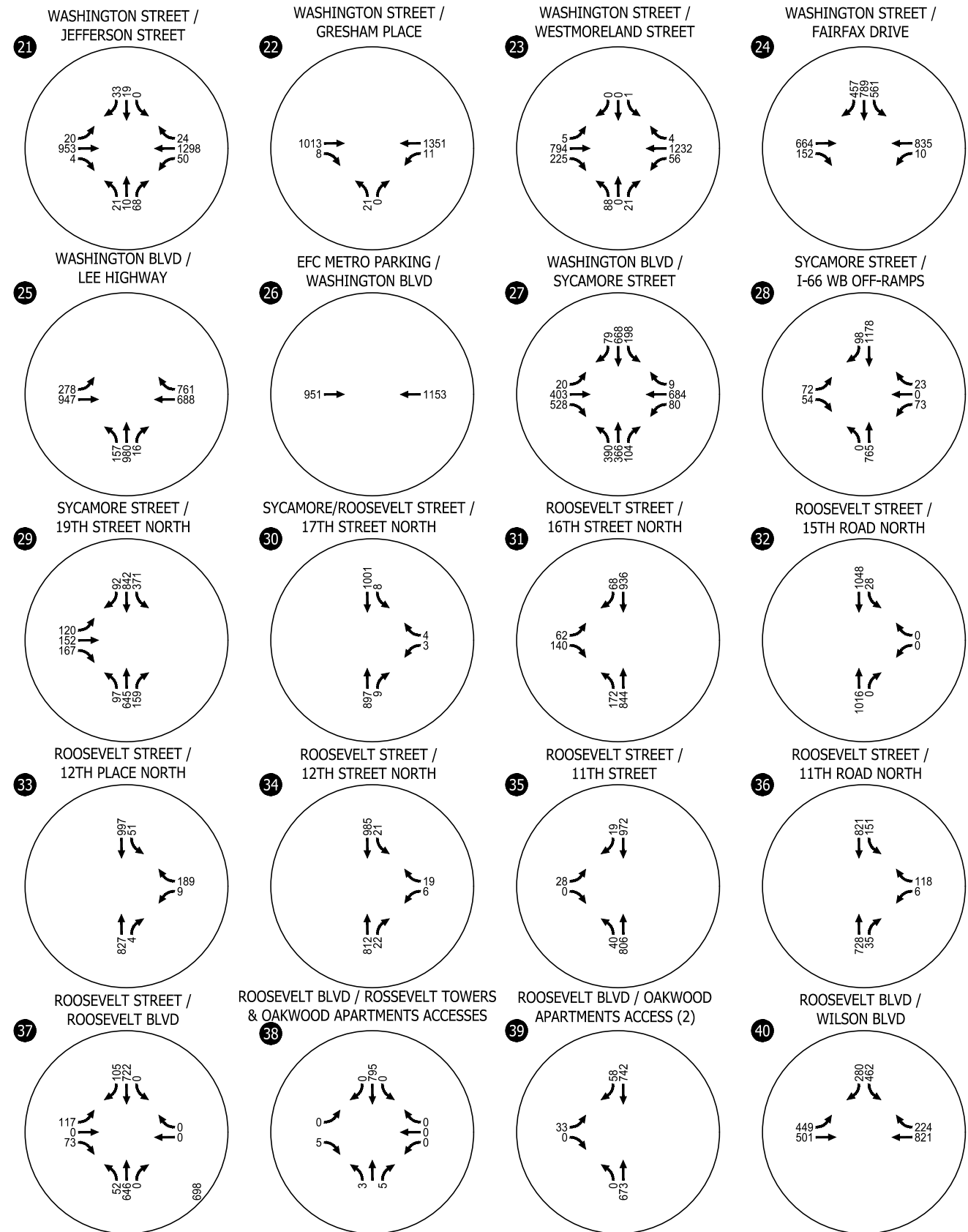
2045 Baseline Traffic Volumes Weekday PM Peak Hour
